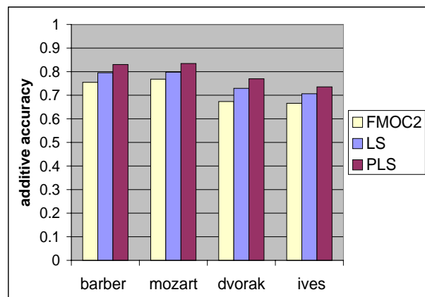
Figure 2: Additive accuracy of FMOC2, LS, and PLS
