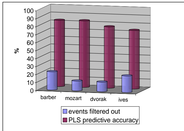
Figure 5: PLS performance vs. percentage of events filtered out of original trace data
