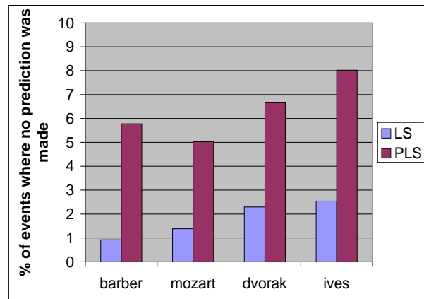
Figure 4: No predictions made by LS and PLS
