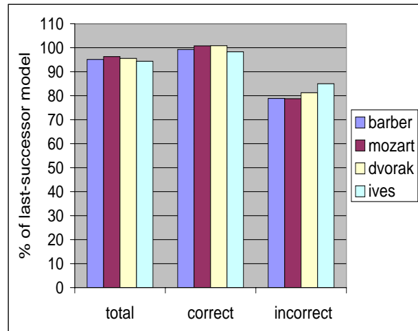
Figure 3: PLS performance normalized by LS in 3 separate categories
