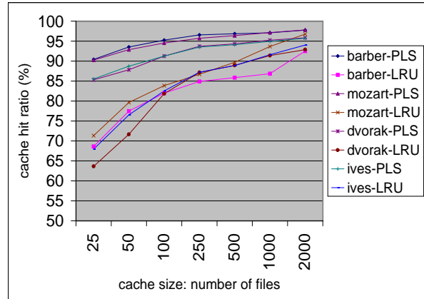
Figure 6: Cache hit ratio of LRU (labelled LRU) and LRU with PLS (labelled PLS)
